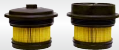
The new WIX 33818 filter kit shown here on the left. (First generation product shown on the right.)
